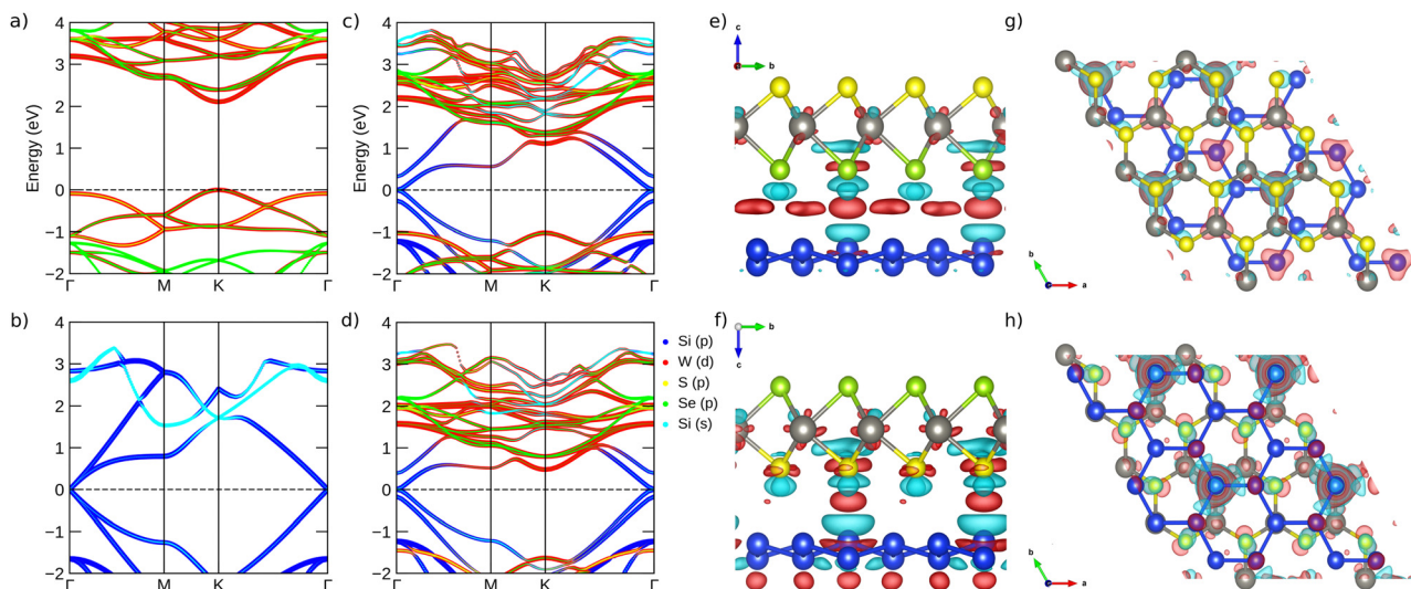
Fig. 2 The band structure projections (using HSE06) considering only orbitals that had a contribution greater than 3% of the maximum total density of states for (a) the WSe 2 Janus geometry, 58 (b) 30 degree rotated silicene, 12 (c) WSe 2 /Si and (d) WSeS/Si; (e)–(g) and (f)–(h) the side and top views of the charge density redistribution for WSe 2 /Si (WSeS/Si); \Delta\rho(\vec{r}) > 0 and \Delta\rho(\vec{r}) < 0 are represented by light red and cyan colors, respectively. Isosurface 0.0006 e Å -3 .
