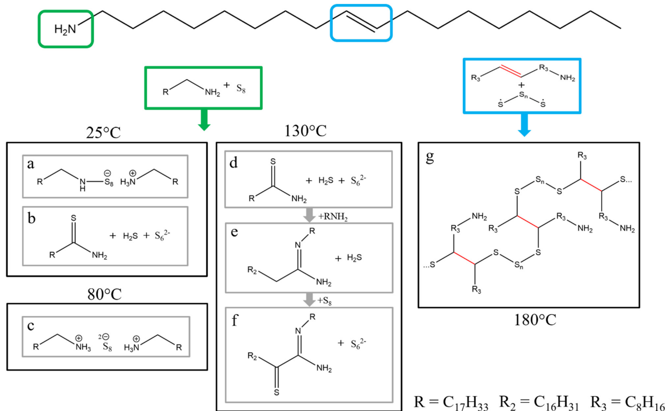
Fig. 1 Molecule structure for oleylamine. Depicted in the green box reaction of elemental sulfur with a primary amine functional group. (a) and (b) reaction at 25^\circ\text{C} reported in ref. 31 (c) reaction at 80^\circ\text{C} reported in ref. 35 (d)–(f) reaction at 130^\circ\text{C} reported in ref. 35. Depicted in the blue box reaction of elemental sulfur with the double bond in oleylamine. (g) polymerization reaction at 180^\circ\text{C} reported from ref. 36.
