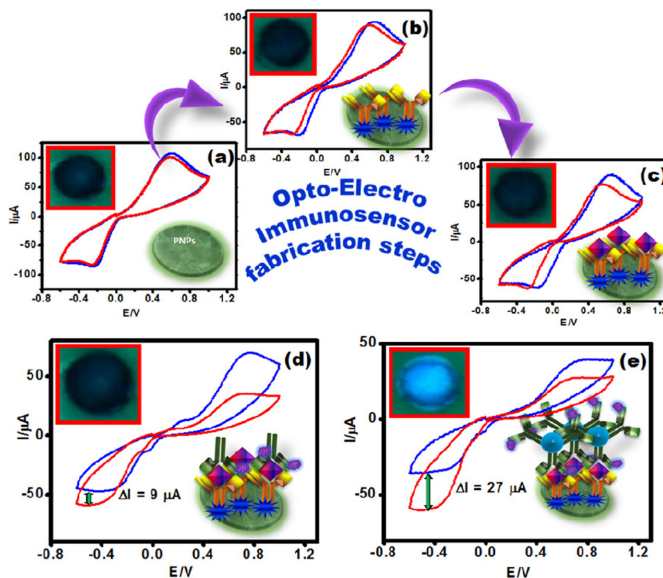
Fig. 5 Cyclic voltammetry during the construction of biosensor (a) SPE-PNPs, (b) SPE-PNPs- \text{PSAAb}_{\text{cap}} , (c) SPE-PNPs- \text{PSAAb}_{\text{cap}} -PSA, (d) SPE-PNPs- \text{PSAAb}_{\text{cap}} -PSA- \text{PSAAb}_{\text{HRP}} , and (e) SPE-PNPs- \text{PSAAb}_{\text{cap}} -PSA- \text{OCDs@PSAAb}_{\text{HRP}} in PBS containing 3 mM HQ (blue) and 4.5 mM \text{H}_2\text{O}_2 (red) at 50 \text{mV s}^{-1} from 1 to -0.6 V vs. Ag/AgCl (inset: corresponding photographic images of sensor circles under UV lamp (FIA)).
