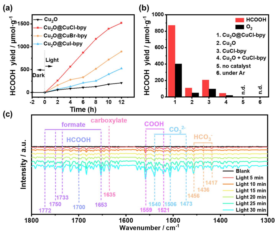
Fig. 4 (a) The yield of HCOOH as a function of the time of visible light illumination over Cu 2 O and Cu 2 O@CuX–bpy. (b) The yield of HCOOH produced with different catalyst and reaction conditions after 6 h of visible light illumination. (c) In situ FTIR spectra for the simulated photo-driven CO 2 reduction process over Cu 2 O@CuCl–bpy.
