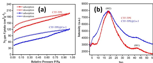
Fig. 2 (a) \text{N}_2 adsorption–desorption isotherm of CTF-TPE and CTF-TPE@Co-3 and (b) PXRD pattern of CTF-TPE and CTF-TPE@Co-3.
