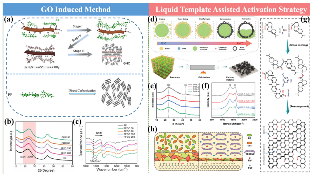
Fig. 7 (a) Proposed formation mechanism of GNCs under different conditions, (b and c) XRD patterns and FTIR spectra of GNCs, (d) diagram for the preparation of "egg puff"-like HC, (e and f) XRD patterns and Raman spectra of SNQLs, (g) diagram of the structure transformation and (h) diagram of SEI in different electrolytes.
