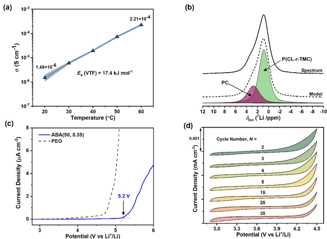
Fig. 3 (a) Temperature-dependence of ionic conductivity for ABA (50, 0.35)/17 wt% LiTFSI. (b) Solid-state {}^7\text{Li} NMR spectrum with peak deconvolution to PC and P(CL- r -TMC) phases. (c) Oxidative stability vs. Li metal and stainless-steel counter electrode measured by LSV at 60 °C, 0.1 mV s ^{-1} scan rate. (d) CV at 0.5 mV s ^{-1} scan rate recorded over 35 cycles.
