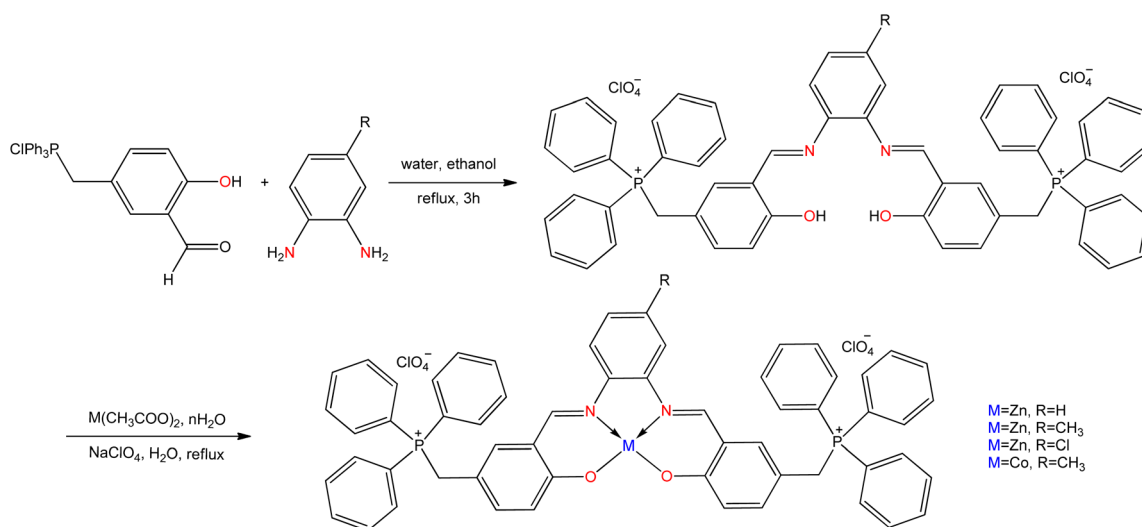
Fig. 16 Synthesis of Schiff base ligand and their metal complexes containing \text{PPh}_3^+ ion.
