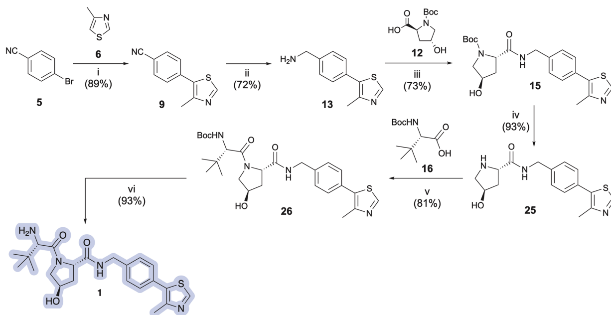
Scheme 2 Initial route used to prepare VH032 ( 1 ). Reagent and conditions: (i) 0.5 mol% Pd-PEPPSI-IPr, K _2 CO _3 (2 equiv.), PivOH (0.3 equiv.), DMA, 125 °C, 2 h; (ii) (a) ( t -Bu) _2 AlBH _4 (1.1 equiv.), THF, 0 °C to r.t., 2 h; (b) 6 M HCl, reflux, 3 h; (iii) HATU (1.3 equiv.), DIPEA (3.5 equiv.), DMF, r.t., 19 h; (iv) (a) CH _2 Cl _2 : TFA (1 : 1), 0 °C, 1 h; (b) NaOH solution until pH = 12.5–13; (v) HATU (1.3 equiv.), DIPEA (3.5 equiv.), DMF, r.t., 18 h; (vi) (a) CH _2 Cl _2 : TFA (1 : 1), 0 °C, 1 h; (b) NaOH solution until pH = 12.5–13.
