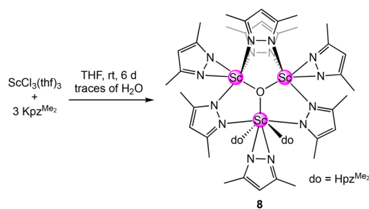
Scheme 6 Synthesis of the oxo-centred cluster [\text{Sc}_3\text{O}(\text{pz}^{\text{Me}_2})_7(\text{Hpz}^{\text{Me}_2})_2] ( 8 ).
