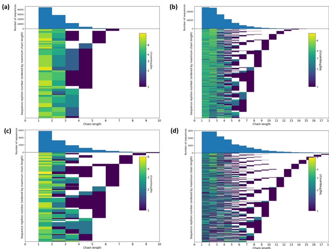
Fig. 6 2D histograms of sequence number against sequence length, with the 1D histogram above, for PLA 20 -PCL 20 (sample 8), where (a) is \epsilon -CL and (b) is L, and for PCL 10 -PLA 20 -PCL 10 (sample 9), where (c) is \epsilon -CL and (d) is L.
