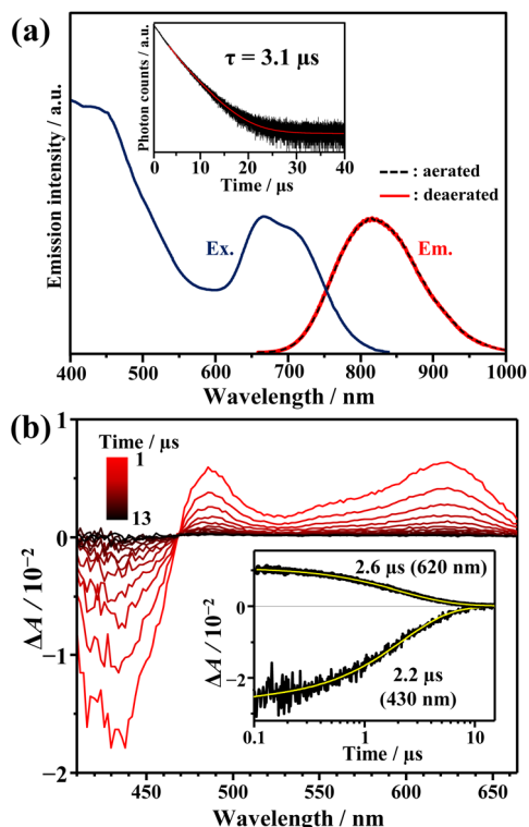
Fig. 2 (a) Excitation (monitored at 850 nm) and emission spectra of AuCu-rod (10 μM) in THF. The inset shows the emission decay curve of AuCu-rod in deaerated THF. (b) Time evolution of transient absorption (TA) spectra, measured for AuCu-rod (47 μM) in deaerated THF (pump at 670 nm). The inset shows the corresponding kinetic traces of the TA signal at 430 and 620 nm.
