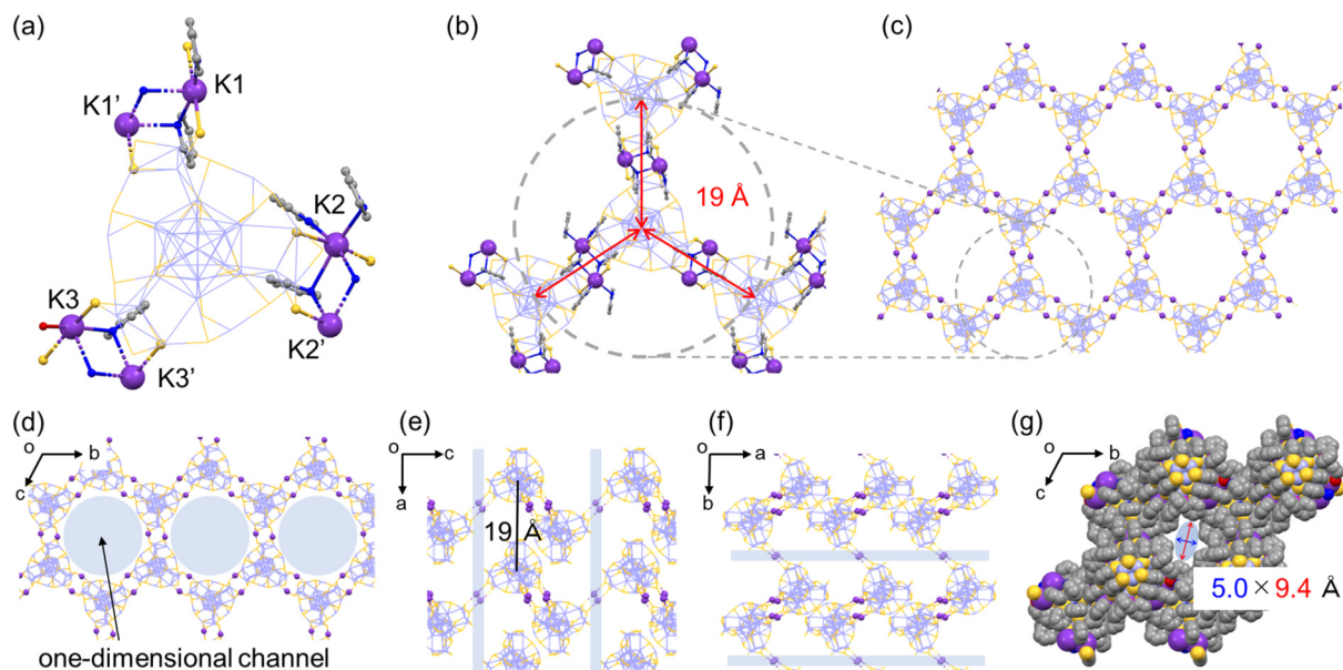
Fig. 4 (a) Unit structure of \text{Ag}_{29}\text{-K}^{\prime} . (b) Packing structure of \text{Ag}_{29}\text{-K}^{\prime\prime} highlighting the bridging style between adjacent NCs. (c) Quasi-2D honeycomb structure composed of \text{Ag}_{29}\text{-K}^{\prime\prime} . Packing structure of \text{Ag}_{29}\text{-K}^{\prime\prime} from the (d) a -axis, (e) b -axis, (f) c -axis. (g) Spacefill packing structure of \text{Ag}_{29}\text{-K}^{\prime\prime} without H atoms. Color code: violet, Ag; yellow, S; purple, K; blue, N; red, O. The solvents and H, C, N and P atoms in NC ligands are omitted for clarity except in (g).
