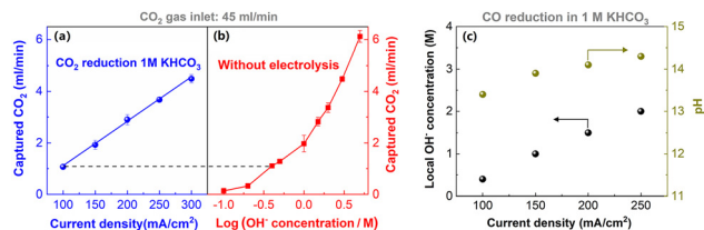
Fig. 7 Comparison of CO 2 capture rates during CO 2 electrolysis at various current densities (a) and for various KOH concentration electrolytes at open-circuit potential (b). (c) The local pH in CO reduction estimated by comparing (c) with (d). This figure has been reproduced from ref. 41 with permission from Royal Society of Chemistry, copyright 2022.
