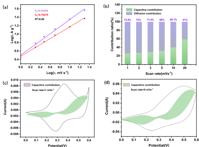
Fig. 8 (a) Kinetic characteristics and reaction mechanism of CoNi 0.5 -MOF/CC electrode; (b) the capacitive contribution of CoNi 0.5 -MOF/CC at different scanning rates; (c and d) the capacitive contribution at 1 mV s -1 and 5 mV s -1 .
