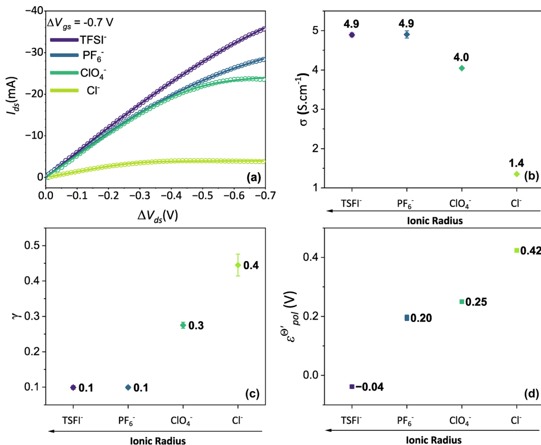
Fig. 5 (a) Output curves (hollow circles) from Flagg (2018), and fitting curves (solid lines) (b) \sigma , (c) \gamma and (d) \epsilon_{pol}^{\ominus'} parameters. Reprinted (adapted) with permission from Flagg et al. (2018). 26 Copyright © 2018, American Chemical Society. All data fittings with R^2 = 0.99 and p -values < 0.05 .
