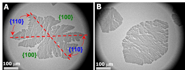
Fig. 4 OM images of a single layer LS-film for a X_{\text{PtBA}} \sim 0.14 PCL/PtBA blend crystalized during an isobaric area relaxation experiment at \Pi \sim (A) 9.5 and (B) 8.5 \text{mN m}^{-1} , respectively.
