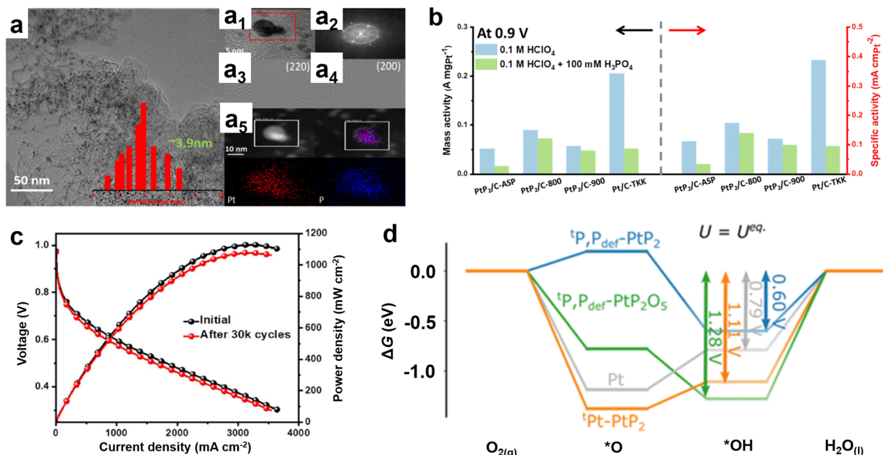
Fig. 9 (a) TEM image of PtP2/C-800 electrocatalysts, the inserted bar graph shows the PtP2 particle size distribution along with the average PtP2 particle size. (a1) HR-TEM image. (a2) FFT patterns of the area enclosed in the red square in (a1). (a5) HAADF images and the corresponding EDX images of (a1). (a3 and a4) Inverse FFT images of the area enclosed in the red square in (a1), where (a3) shows the distribution of 220 planes while (a4) shows the presence of 200 planes. (b) Mass and specific activity profiles; (c) long-term durability tests of PtP2/C-800; (d) free energy diagram for the ORR on four different active site models constructed from the (111) surfaces. Reprinted with permission from ref. 53. Copyright 2023, Royal Society of Chemistry.
