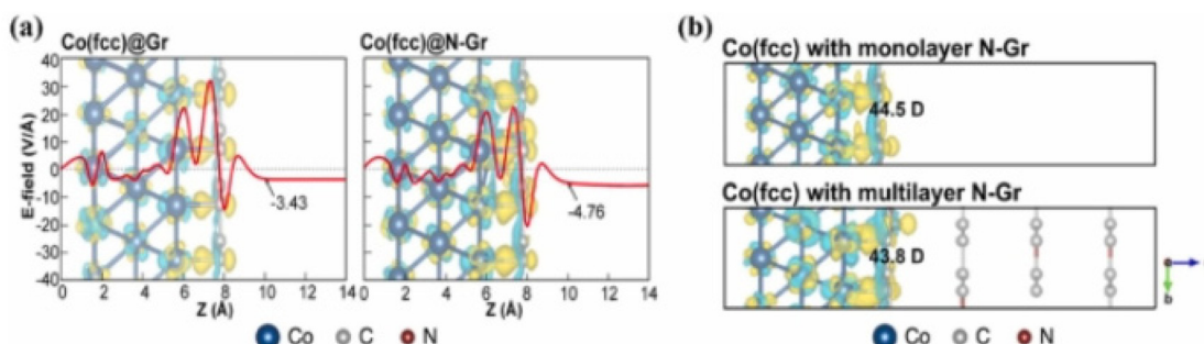
Fig. 20 (a) Electric field calculated for (a) Co(fcc)Gr and Co (fcc)NGr in z-direction as a function of position with different charge density and (b) graphical representation of charge density difference along z-axis with monolayer and multilayer N-Gr over Co(fcc), where the numerical values present in the different graphs represent the dipole moment. Blue and yellow regions represent the electron accumulation and depletion regions, respectively. Reprinted with permission from ref. 174. Copyright 2022, Elsevier.
