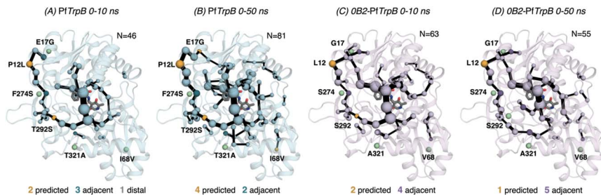
Fig. 5 Evolution of the SPMs along the MD time. The number of identified conformationally relevant positions ( N ) is increased from 46 to 81 in the case of (A and B) PflTrpB , and slightly decreased from 63 to 55 in (C and D) OB2-PflTrpB . The size of spheres and the thickness of edges in the SPM plots are weighted according to their importance for the conformational dynamics of the enzyme: those pairs of residues that have a higher contribution to the conformational dynamics are represented with a thicker edge and larger sphere. All SPM graphs have been generated using the default settings: a threshold of 6.0 Å for the distance matrix, and a 0.3 for the significance threshold.
