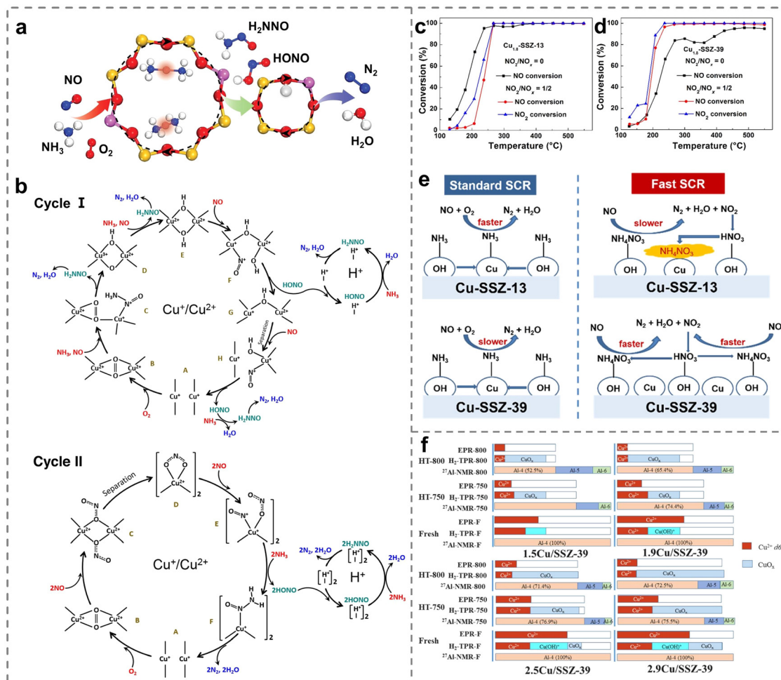
Fig. 4 (a) The reaction route in the multisite fashion for \text{NH}_3\text{-SCR} over Cu-CHA. (b) Two possible reaction mechanisms of \text{NH}_3\text{-SCR} . Copied with permission from ref. 77. Copyright 2020, American Chemical Society. (c) and (d) \text{NH}_3\text{-SCR} activity over (c) \text{Cu}_{1.8}\text{-SSZ-13} and (d) \text{Cu}_{1.8}\text{-SSZ-39} catalysts. Copied with permission from ref. 78. Copyright 2020, American Chemical Society. (e) The influences of \text{NO}_2 on \text{NH}_3\text{-SCR} processes on Cu-SSZ-13 and Cu-SSZ-39. Copied with permission from ref. 79. Copyright 2021, Elsevier. (f) The contents of Al and Cu species quantified on Cu/SSZ-39 zeolites. Copied with permission from ref. 79. Copyright 2021, Elsevier.
