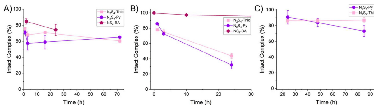
Fig. 7 Kinetic inertness of [\text{H}^{197\text{m/g}}\text{Hg}][\text{Hg}(\text{N}_2\text{S}_4\text{-Py})]^{2+} and [\text{H}^{197\text{m/g}}\text{Hg}][\text{Hg}(\text{N}_2\text{S}_4\text{-Thio})]^{2+} against (A) human serum, (B) glutathione with comparison to the formerly reported \text{NS}_4\text{-BA} and (C) stable biologically relevant metals ( \text{ZnCl}_2 , \text{FeCl}_3 , \text{CuCl}_2 , \text{MgCl}_2 and \text{CoCl}_2 ) at 37^\circ\text{C} ( n = 3 ) over time. [\text{H}^{197\text{m/g}}\text{Hg}][\text{Hg}(\text{NS}_4\text{-BA})]^{2+} stability data are reproduced from Randhawa et al. 10
