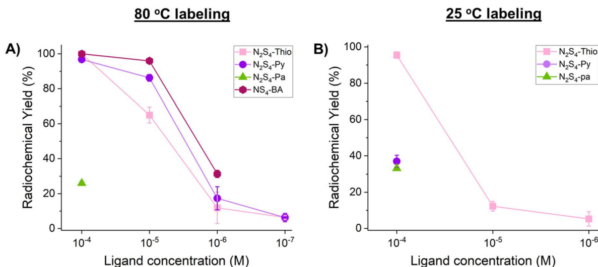
Fig. 6 Non-isolated radiochemical yields (RCYs) for [ 197m/g Hg]HgCl 2 (~1 MBq) radiolabeling of N 2 S 4 -Py, N 2 S 4 -Thio and N 2 S 4 -Pa 2- (1 M NH 4 OAc, pH 7), at various ligand concentrations at 80 °C (A) and 25 °C (B) (1 h reaction time, 100 μL reaction, and n = 3). [ 197m/g Hg][Hg(NS 4 -BA)] 2+ 80 °C labeling data are reproduced from Randhawa et al. 10
