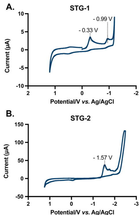
Fig. 3 Cyclic voltammograms of STG compounds (5 mM) in DMSO with [\text{N}(\text{Bu})_4\text{PF}_6] as supporting electrolyte. Potentials are shown vs. \text{Ag}/\text{AgCl} . (A) Voltammogram of STG-1 showing two reduction events at -0.33 V and -0.99 V. (B) Voltammogram of STG-2 showing one reduction event at -1.57 V. Data collected with a glassy carbon working electrode and Pt counter electrode.
