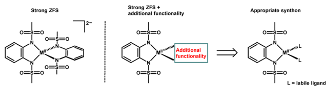
Scheme 1 Conceptual approach: a modular route to functional heteroleptic structures requires appropriate synthons.
