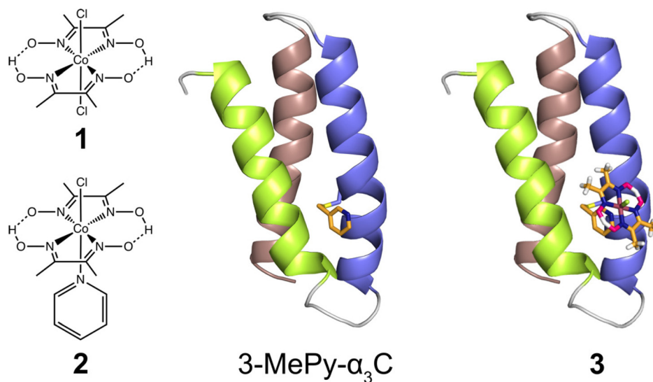
Fig. 1 Left: Cobaloximes used in the present study: [Co(dmgH) 2 Cl 2 ] (1), and [Co(dmgH) 2 (py)Cl] (2). Center: A structural model of 3-MePy-α 3 C (3-MePy = 3-methyl pyridine) based on the related protein system 2MP-α 3 C (2MP = 2-mercaptophenol), RSCB PDB ID 2LXY. 17 Sidechains are omitted for clarity. Helix 1, 2, and 3 of the α 3 scaffold is shown in lime green, blue, and taupe, respectively. Right: A model of the artificial hydrolase, 3, based on 3-MePy-α 3 C.
