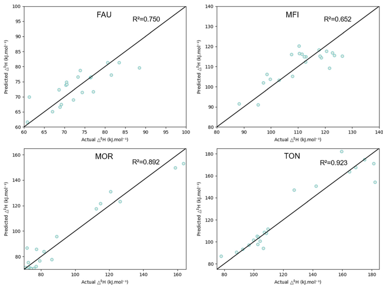
Fig. 11 Parity plots of the predicted and calculated activation enthalpy by the modified group additive model with pore confinement descriptor ( \text{mGAV} + \Delta(\sum d^{-1})_{MM} ) for the four different zeolites. The model trained and evaluated on all reactions included in this work.
