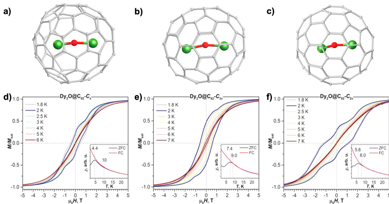
Fig. 6 Molecular structures of \text{Dy}_2\text{O}@\text{C}_{82} (a), \text{Dy}_2\text{O}@\text{C}_{3v}(8)-\text{C}_{82} (b) and \text{Dy}_2\text{O}@\text{C}_{2v}(9)-\text{C}_{82} (c). Magnetic hysteresis curves of \text{Dy}_2\text{O}@\text{C}_{82} (d), \text{Dy}_2\text{O}@\text{C}_{3v}(8)-\text{C}_{82} (e) and \text{Dy}_2\text{O}@\text{C}_{2v}(9)-\text{C}_{82} (f) in the range of 1.8–7 K using a field sweep rate of 2.9 \text{ mT s}^{-1} . The insets represent their corresponding ZFC/FC curves at an applied magnetic field of 0.2 T with a temperature sweep rate of 5 \text{ K min}^{-1} . Reproduced from ref. 102.
