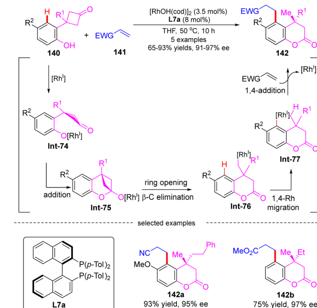
Scheme 40 Rhodium-catalyzed cascade reaction of 3-(2-hydroxyphenyl)cyclobutanones with electron-deficient alkenes.
