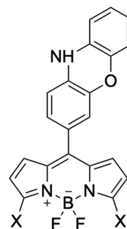
Fig. 4 Chemical structures of \text{BDP-PXZ} derivatives with substituent groups X , as X = \text{Me} , \text{NO}_2 , and \text{NH}_2 in potential energy curve analysis, and X = \text{F} , \text{Cl} , \text{NH}_2 , \text{OMe} , \text{Me} , \text{H} , \text{CF}_3 , \text{Ac} , \text{CHO} , \text{CN} , and \text{NO}_2 in Hammett substituent constant analysis.
