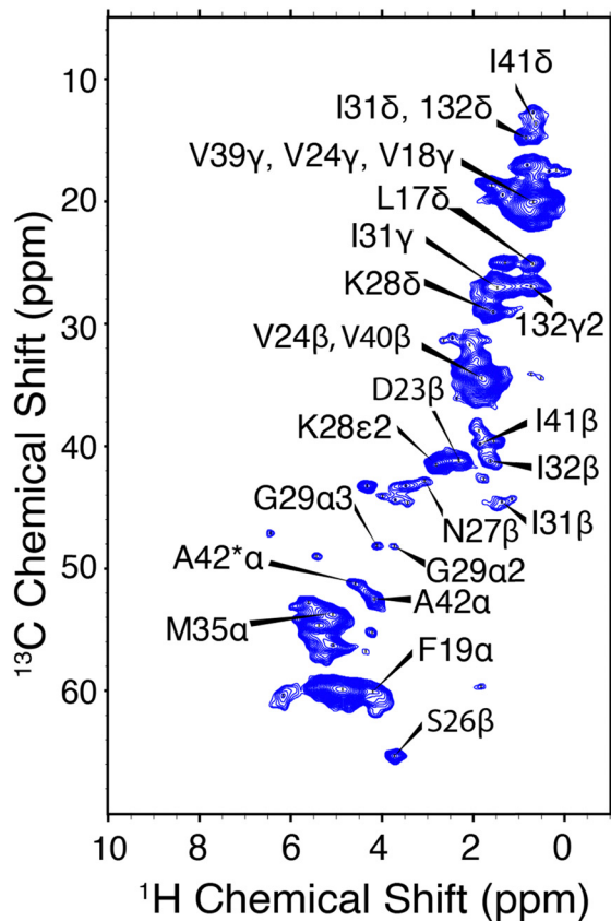
Fig. 4 hCH correlations of E22G-A \beta_{1-42} amyloid fibrils. The assigned chemical shifts are consistent with a structure similar to A \beta_{1-42} . \omega_r/2\pi = 90 kHz and \omega_{\text{DH}}/2\pi = 800 MHz. Mixing times and other spectral acquisition parameters are tabulated in Table S2 (ESI \dagger ).
