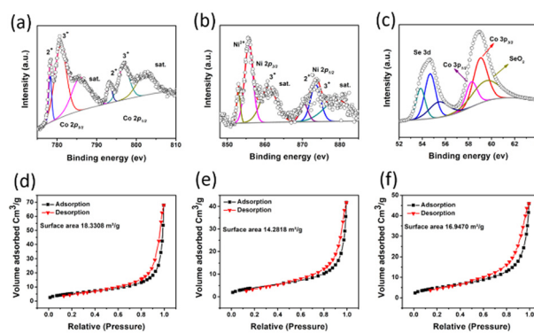
Fig. 4 X-ray photoelectron spectroscopy for (a) Co; (b) Ni; (c) Se; BET surface area for (d) 10% Ni-doped (\text{Ni},\text{Co})_{0.85}\text{Se} ; (e) undoped \text{Co}_{0.85}\text{Se} ; and (f) 15% Ni-doped (\text{Ni},\text{Co})_{0.85}\text{Se} .
