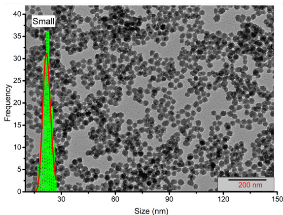
Fig. 2 TEM image and silica core diameter distribution for sample NPs-Ru(bpy) 2 bpy 3 2+ (small): d_c = (22 \pm 2) nm. Other sample images are reported in the ESI.†
