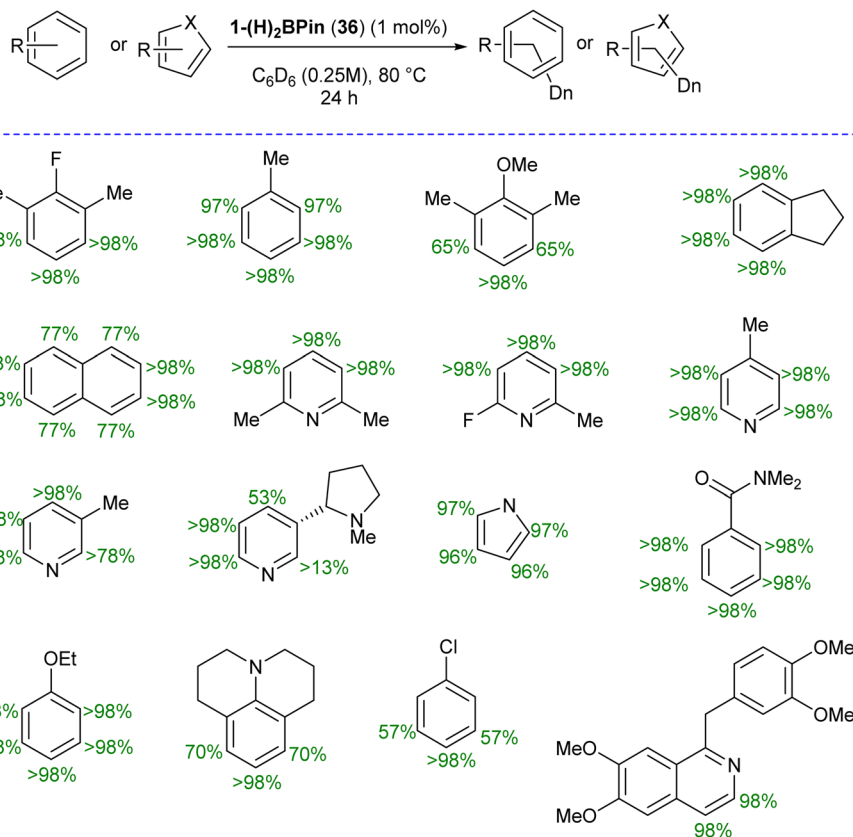
Scheme 14 Substrate scope for HIE reaction using 36 .
