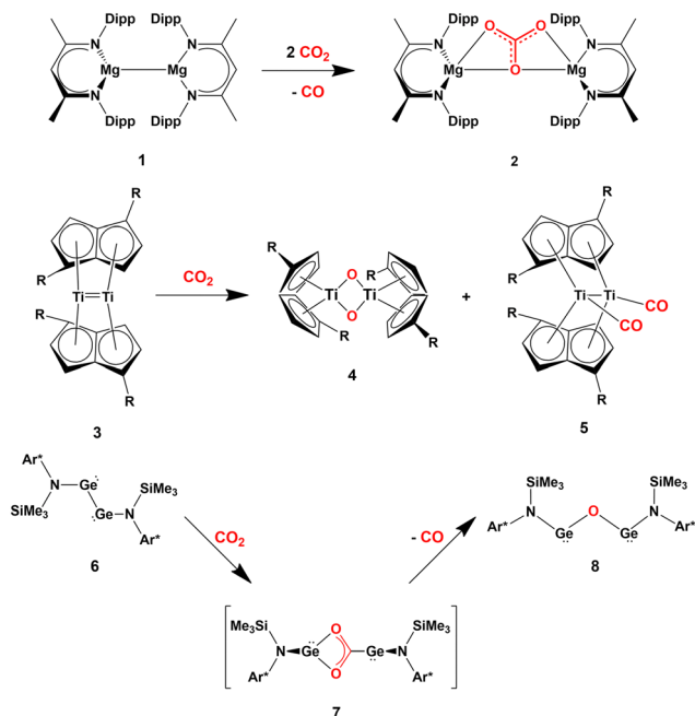
Scheme 1 Relevant examples of cooperative CO 2 activation with s- ( 1 ), d- ( 3 ) and p-block ( 6 ) homobinuclear compounds featuring apolar E–E bonds. (R = Si i Pr 3 ; Ar* = C 6 H 2 (C(H)Ph 2 ) 2 Me–2,6,4).
