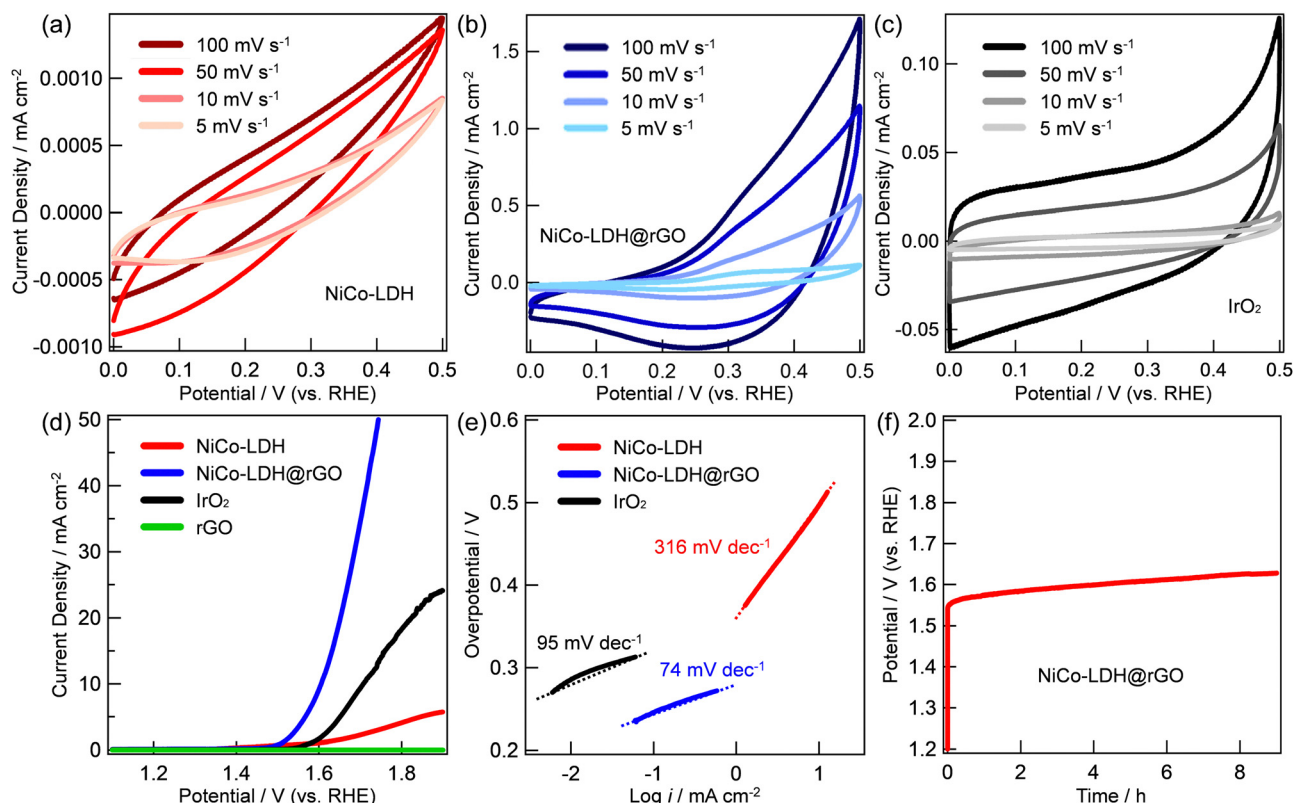
Fig. 2 Electrocatalytic OER performance of the prepared electrocatalyst. CV curves conducted at voltages ranging between 0 and 0.5 V and scan rates ranging from 5 to 100 \text{ mV s}^{-1} of (a) NiCo-LDH, (b) NiCo-LDH@rGO, and (c) \text{IrO}_2 . (d) Linear sweep voltammetry polarization curves of rGO, NiCo-LDH, NiCo-LDH@rGO, and \text{IrO}_2 at 1 M KOH during OER testing. (e) Tafel plot of NiCo-LDH, NiCo-LDH@rGO, and \text{IrO}_2 towards the OER, and (f) chronopotentiometry (time-dependence of the potential) for NiCo-LDH@rGO conducted under 1 M KOH at 5 \text{ mA cm}^{-2} indicating the stability.
