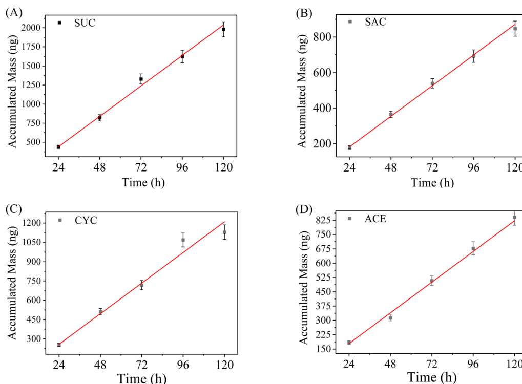
Fig. 2 Accumulated masses ( M ) of SUC (A), SAC (B), CYC (C), and ACE (D) by WAX-XDA1-DGT devices deployed in 2 L of 50 \mu\text{g L}^{-1} AS solutions containing 0.01 \text{ M NaCl} ( 23 \pm 0.4 °C). The solid red lines demonstrate the theoretical lines predicted by the equation: M = DCAT/\Delta g ( C is the concentration of the solution, A is the exposed window area of the DGT, t represents the deployment duration and \Delta g is the diffusive layer thickness.) Error bars: 1 SD ( n = 3 ). SUC: Sucralose, SAC: Saccharin, CYC: Cyclamate, ACE: Acesulfame.
