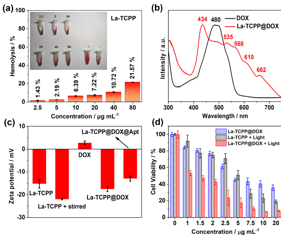
Fig. 3 (a) Effect of different concentrations of La-TCPP on the hemolysis rate of red blood cells after 1 h of incubation. (b) UV-vis absorption of DOX and La-TCPP@DOX. (c) Zeta potential of La-TCPP, La-TCPP + stirred, DOX, La-TCPP@DOX, and La-TCPP@DOX@Apt. (d) Relative viability of 4T1 cells treated with La-TCPP@DOX, La-TCPP + light, and La-TCPP@DOX + light. Laser conditions: 660 nm, 100 \text{ mW cm}^{-2} , and 15 min.
