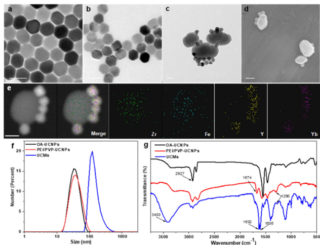
Fig. 1 TEM images of (a) UCNP (NaYF 4 :25% Yb 3+ , 0.9% Tm 3+ , 0.6% Nd 3+ ), (b) dual-ligand PEI/PVP modified UCNP, and (c) UCMPs. (d) SEM images of UCMPs. (e) Dark-field TEM images and the corresponding area-elemental mapping of UCMPs, including Zr, Fe, Y and Yb. (f) The statistical data showing the size distributions of OA-UCNPs, PEI/PVP-UCNPs and UCMPs. (g) FT-IR spectra for OA-UCNPs, PEI/PVP-UCNPs and UCMPs. The scale bars indicate 50 nm in all the tested cases.
