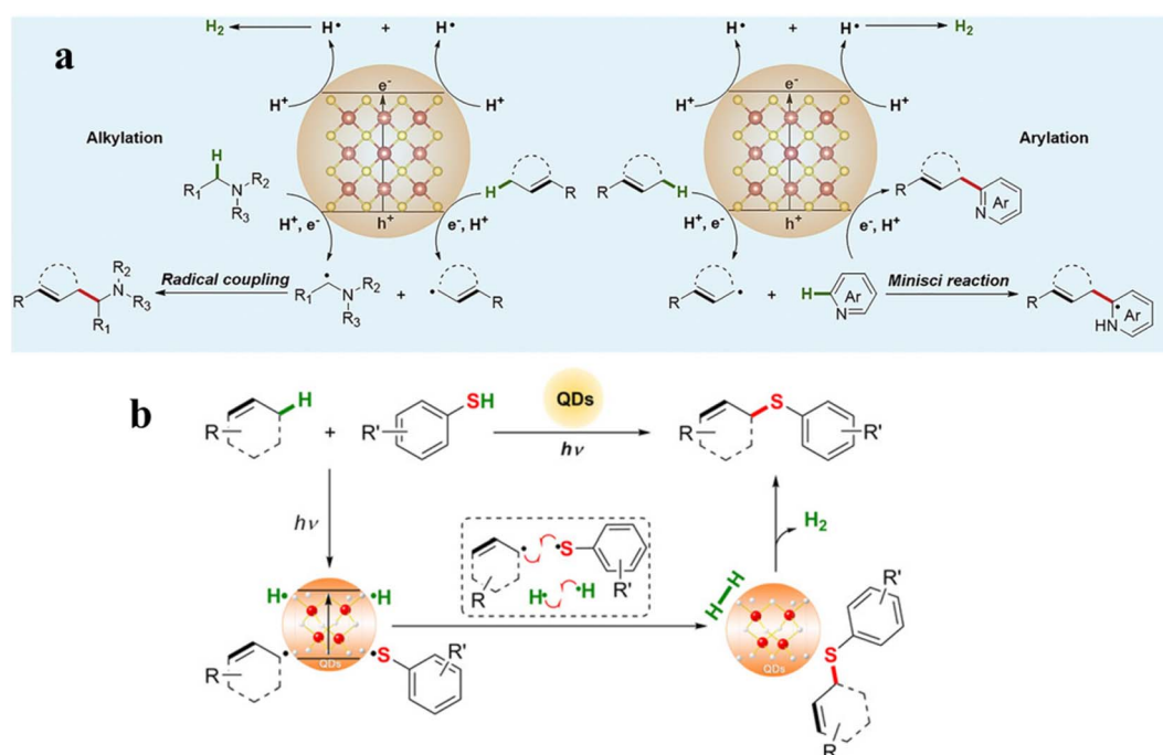
Fig. 10 (a) Alkylation and arylation of an allylic \text{C}(\text{sp}^3)\text{--H} bond. Reprinted with permission from ref. 122. (b) Direct activation of an allylic C–H bond to form a C–S bond. Reprinted with permission from ref. 123.
