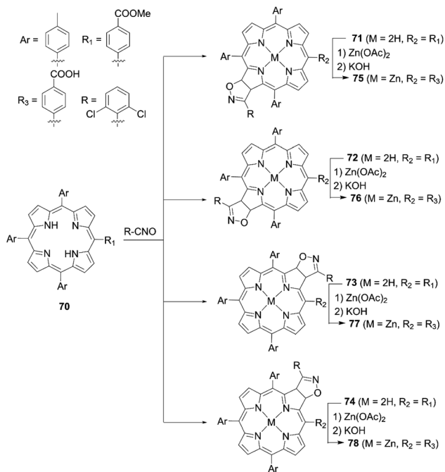
Scheme 16 Syntheses of 75–78.
