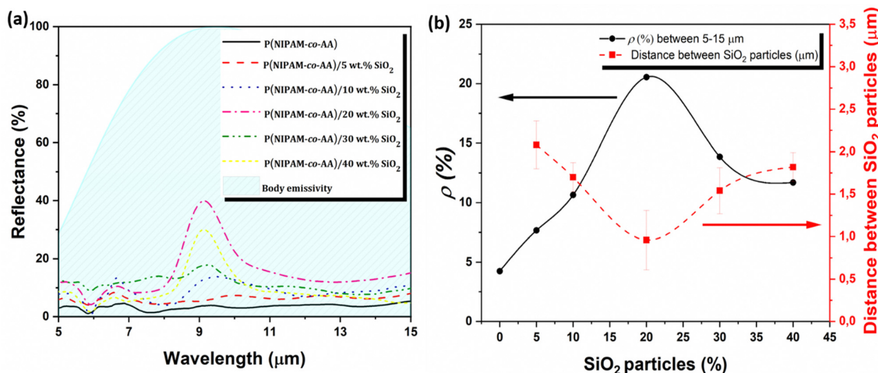
Fig. 1 (a) Evolution of the reflectance in the 5–15 \mu\text{m} range of the PNIPAM-based hydrogel composites as a function of the \text{SiO}_2 content, with the human body emissivity at a skin temperature of 34 ^\circ\text{C} . (b) Percentage of infrared radiation emitted by the human body that is reflected by the PNIPAM-based hydrogel composites (black circles) as well as the distance between the \text{SiO}_2 particles (red squares) with respect to the \text{SiO}_2 content.
