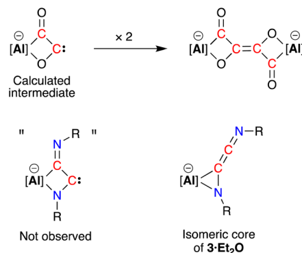
Fig. 6 Calculated carbene intermediate in the formation of the [(\text{CO})_4]^{4-} ligand, with the analogous dimerised isocyanide (not observed) and isomeric core of 3 \cdot \text{Et}_2\text{O} .
