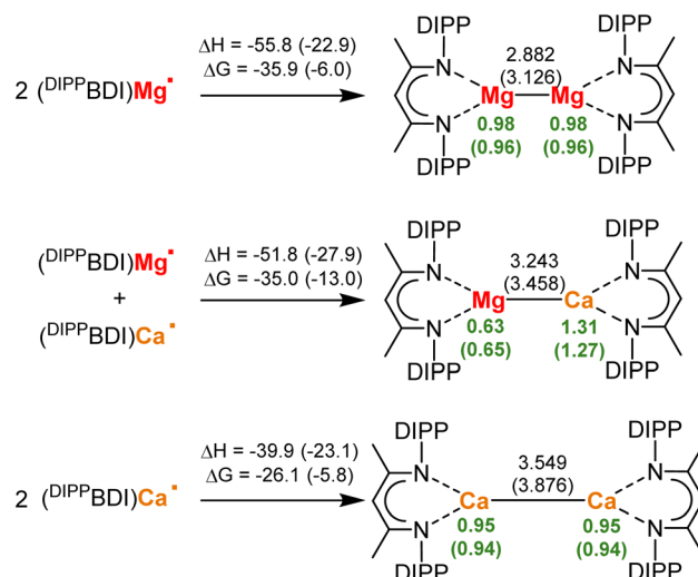
Scheme 2 Formation of homo- and hetero-metallic (^{\text{DIPeP}}\text{BDI})\text{Ae–Ae} ( \text{Ae} = \text{Mg} or \text{Ca} ). Enthalpies and Gibbs free energies at 298 K in kcal mol −1 , Ae–Ae distances in Å and NPA charges in green; B3PW91/def2TZVP//def2SVP with dispersion correction (GD3BJ). Values in brackets relate to calculations without dispersion corrections.
