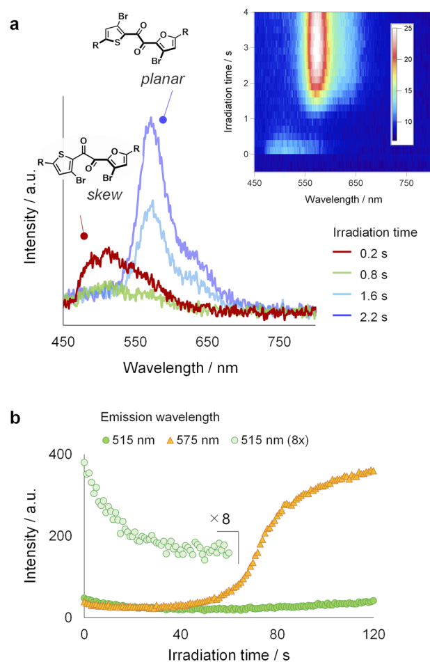
Fig. 3 Time course of (a) photoluminescence spectra and (b) luminescence intensity ( \lambda_{\text{em}} = 515 nm and 575 nm) of SO crystal during continuous UV irradiation. Note that crystal size and light source for panels (a) and (b) are different.
