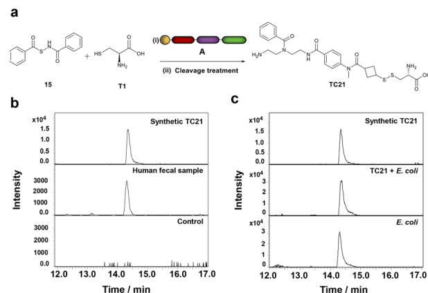
Fig. 4 Validation of cysteine persulfide in biological samples. (a) Synthesis of cysteine persulfide-probe conjugate TC21 . Reaction conditions. (i) 15 , T1 , probe A , THF, and PBS; (ii) 1,3-dimethylbarbituric acid, triphenylphosphine, Pd(OAc) 2 , and THF. (b) Comparison of extracted ion chromatograms (EICs) of synthetic TC21 and natural cysteine persulfide in the human fecal sample and the control sample. (c) Co-injection experiment: EIC comparison of the synthetic TC21 , the co-injected synthetic TC21 and the E. coli lysate as well as the metabolite in E. coli .
