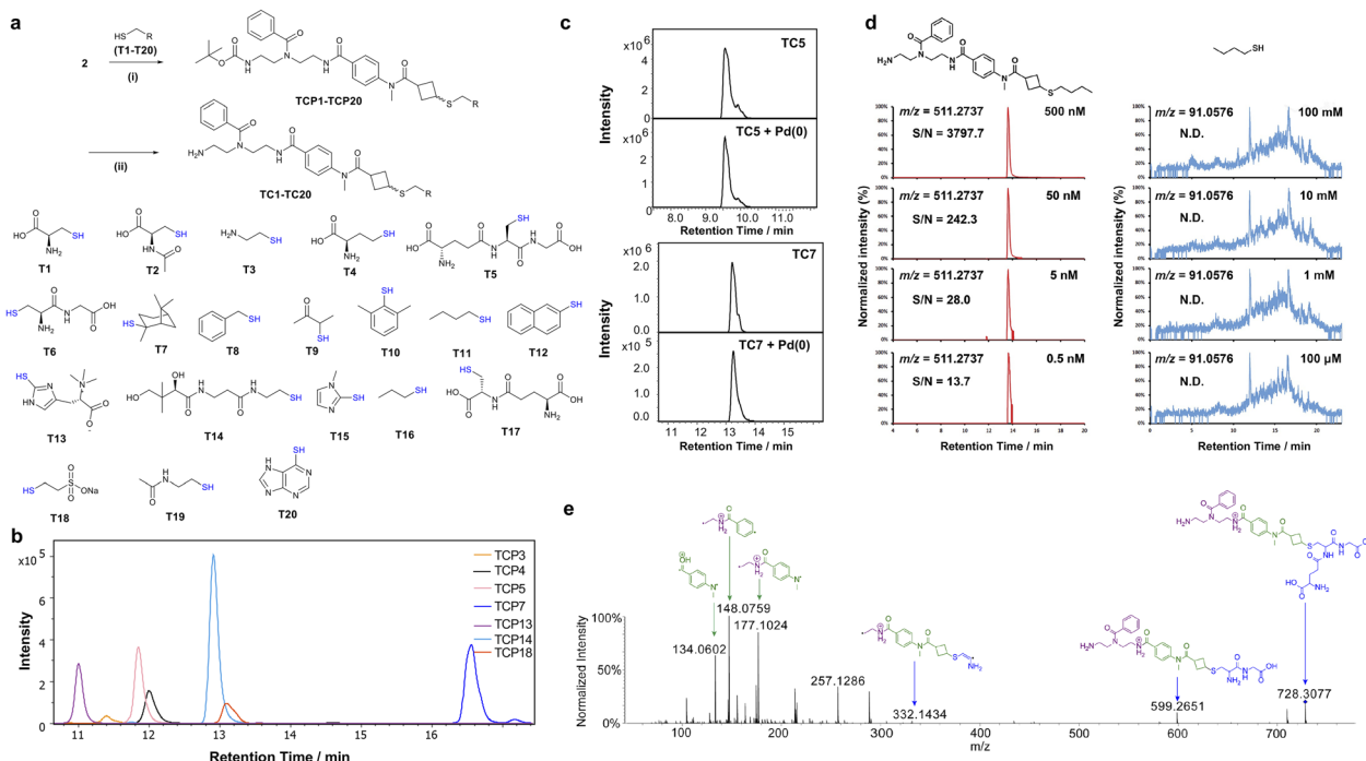
Fig. 2 Capture efficiency and analysis of the conjugated thiols. (a) Reactivity of simplified probe 2 with thiols T1 – T20 . Reaction conditions: (i) 2, thiol ( T1 – T20 ), Et 3 N, DMF or K 2 CO 3 , and DMF/H 2 O (1 : 1); (ii) TFA. (b) Representative mass spectrometric extracted ion chromatograms of 7 selected thiol conjugates that were successfully captured (TCP3, TCP4, TCP5, TCP7, TCP13, TCP14, and TCP18) after treatment with 2. Conditions: Et 3 N in DMF at 28 °C for 16 h. (c) Stability of two Boc-protected thiol conjugates (TC5 (glutathione) and TC7 (2,3,10-mercaptopyranine)) after Pd(0) treatment at 25 °C for 18 h. Top: extracted ion chromatograms (EICs) of the corresponding thiol conjugate before Pd(0) treatment. Bottom: unchanged EICs after Pd(0) treatment. (d) EICs of the LOD measurements comparing 1-butanethiol with conjugated 1-butanethiol. (e) MS/MS fragmentation of the thiol glutathione conjugate TC5 with CID (30–75 eV).
