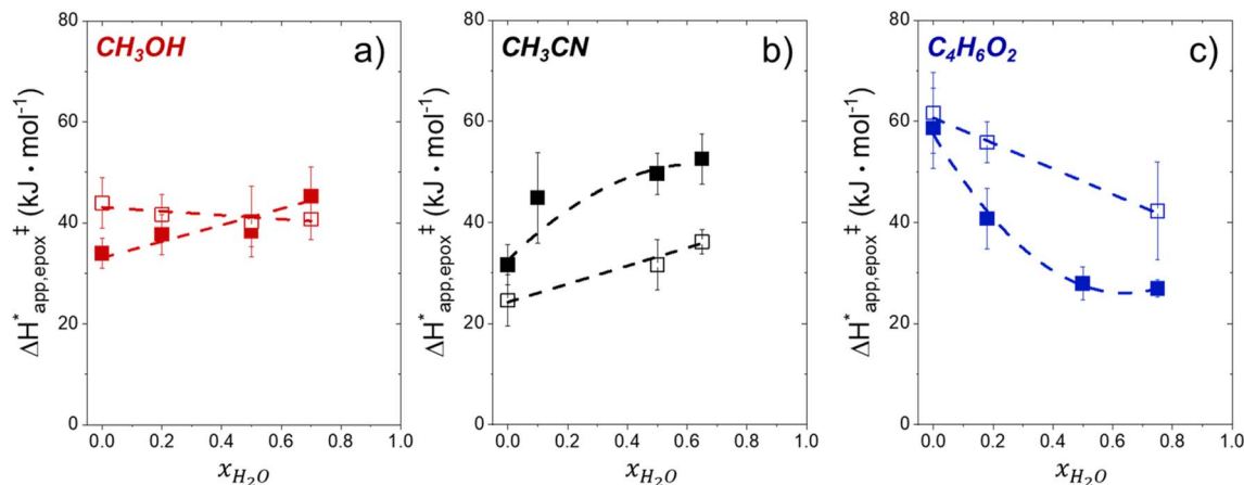
Fig. 5 \Delta H^*_{app,epox} values for \text{C}_6\text{H}_{12} epoxidation (1 mM \text{C}_6\text{H}_{12} , 10 mM \text{H}_2\text{O}_2 , 308–333 K) as a function of x_{H_2O} in mixtures of (a) \text{CH}_3\text{OH} (■, □), (b) \text{CH}_3\text{CN} (■, □), and (c) \text{C}_4\text{H}_6\text{O}_2 (■, □) with \text{H}_2\text{O} over Ti-BEA-OH (solid) and Ti-BEA-F (hollow).
