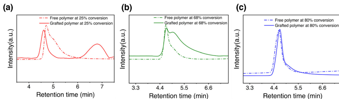
Fig. 4 SEC traces for free polymers from solution (FP) and grafted polymers (GP) from polystyrene grafted silica synthesized via ECPS (PSRHA) at (a) 25% conversion, (b) 68% conversion, and (c) 80% conversion. The free polymers were obtained by precipitating the decant in cold methanol after centrifugation and the grafted polymers were cleaved by transesterification of polystyrene grafted silica synthesized via ESCP using p -toluenesulfonic acid and methanol in toluene. The broader dispersity and multiple populations of grafted polystyrene than that of the single population of free polymers was observed due to the ability of surface nitrene functionalities to capture and terminate the growing polymer radicals at any stage of propagation. The molecular weight of grafted polystyrene observed at 25% conversion was 85\,000\text{ g mol}^{-1} , with respect to the 38\,000\text{ g mol}^{-1} of free polymers, which confirms the potential of nitrene functionalities to capture two polymer radicals.
