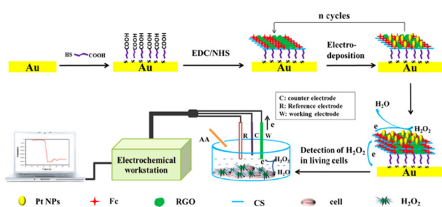
Fig. 8 Analytical principle for the detection of H 2 O 2 in living cells with the nonenzymatic biosensor based on PtNPs/RGO-CS-Fc nanohybrids (reprinted from ref. 100 with permission from Elsevier).
