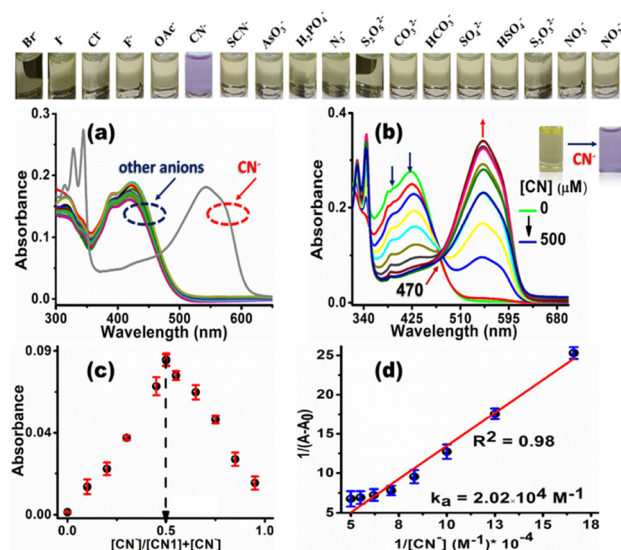
Fig. 5 (a) UV/Vis absorption spectra of CN1 (10 μM) in an 8:2 (v/v) DMSO/water mixture in the presence of different anionic solutions (5 equiv.), where the inset above (a and b) shows the naked eye colorimetric response of the CN1 solution in the presence of each anion. (b) Variation in the UV/Vis absorption spectra of CN1 (10 μM) in an 8:2 (v/v) DMSO/water mixture with increasing aqueous [CN⁻], where the inset shows the naked eye colorimetric response of the CN1 solution in the presence of CN⁻. (c) Job's continuous variation plot and (d) Benesi-Hildebrand plot of CN1 (10 μM) with increasing [CN⁻].
