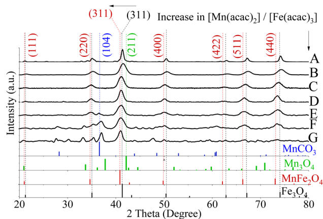
Fig. 2 XRD patterns for fcc lattice of Fe 3 O 4 (A) and Mn x Fe 3-x O 4 NPs where [\text{Mn}(\text{acac})_2]/[\text{Fe}(\text{acac})_3] were 0.14 (B), 0.33 (C), 0.6 (D), 1 (E), 1.66 (F), 3 (G). The horizontal arrow pointed out the shifting in the peak of 311 from the reference Fe 3 O 4 (PDF card no. 01-089-0688) towards the lower diffraction angle of MnFe 2 O 4 (PDF card no. 00-010-0319) in response to the increase in [\text{Mn}(\text{acac})_2]/[\text{Fe}(\text{acac})_3] . A secondary phase of MnCO 3 (Reference ICDD PDF card no. 00-044-1472) was found for NPs prepared from 1 \leq [\text{Mn}(\text{acac})_2 \text{ or } 3]/[\text{Fe}(\text{acac})_3] \leq 3 (E)–(G). The synthesis temperature for all NPs was 250 °C. The vertical arrow indicated the gradual increase in [\text{Mn}(\text{acac})_2]/[\text{Fe}(\text{acac})_3] from (A)–(G) Mn 3 O 4 (PDF card no. 01-080-0382).
