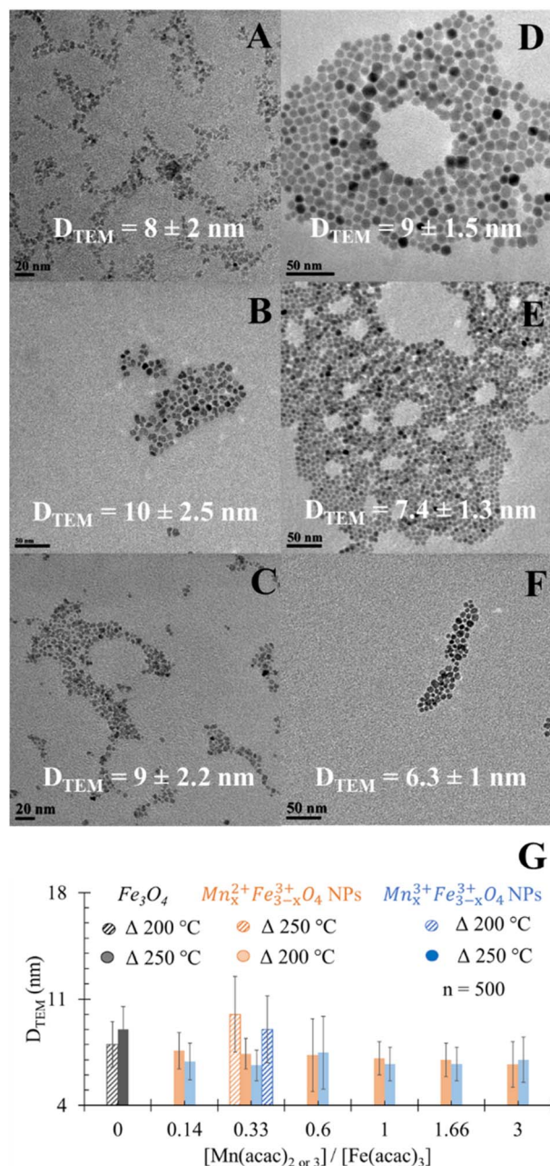
Fig. 1 TEM images for the spherical (A) undoped Fe 3 O 4 NPs, (B) Mn x Fe 3-x O 4 of precursor ratio [\text{Mn}(\text{acac})_2]/[\text{Fe}(\text{acac})_3] = 0.33 , (C) [\text{Mn}(\text{acac})_3]/[\text{Fe}(\text{acac})_3] = 0.33 prepared at 200 °C as reaction temperatures, (D) undoped Fe 3 O 4 NPs and (E) and (F) Mn x Fe 3-x O 4 NPs prepared with the same precursor ratio but at 250 °C. (G) Impact of reaction temperatures on D_{\text{TEM}} of Mn x Fe 3-x O 4 NPs prepared from [\text{Mn}(\text{acac})_2]/[\text{Fe}(\text{acac})_3] = 0.33 . * P < 0.05 .
